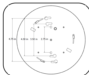
6" Junction box
