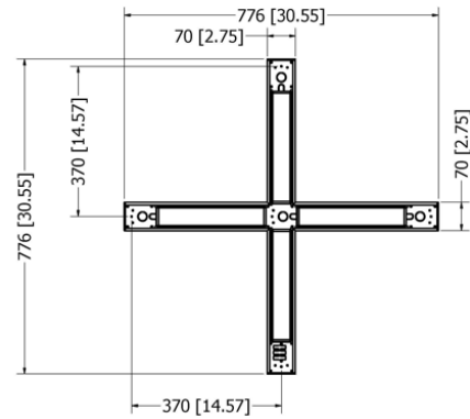
X-SHAPE AE-SF-G5-1-1-X
