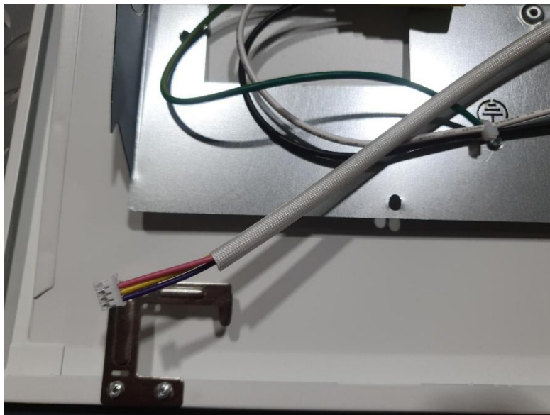
2. Locate the dimming wires (pink and Purple) and the 12v (yellow)
