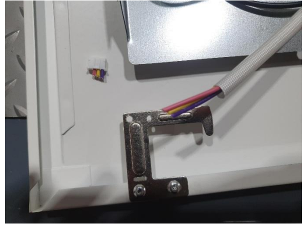
3. Cute the three wires
