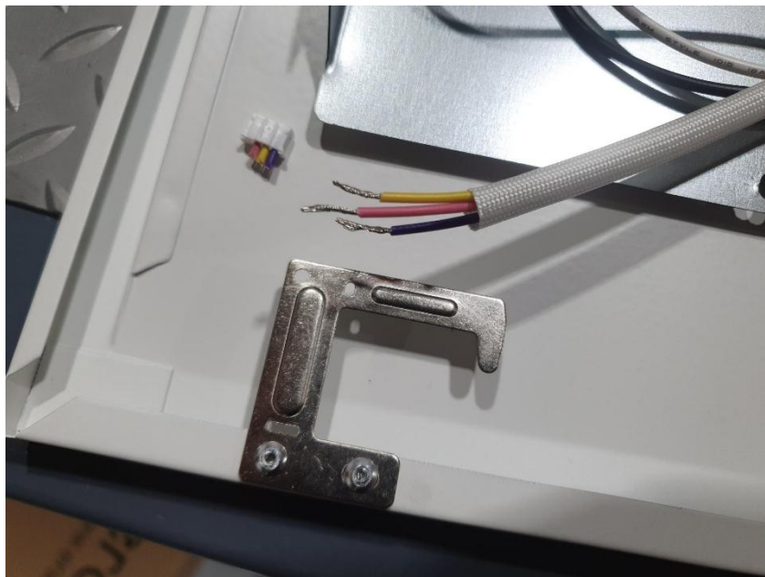
4. Strip the wires and you can use the purple (+ve) and pink wires (-ve) for dimming
