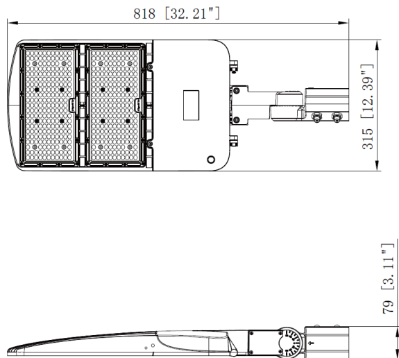
Slip Fitter mounting
